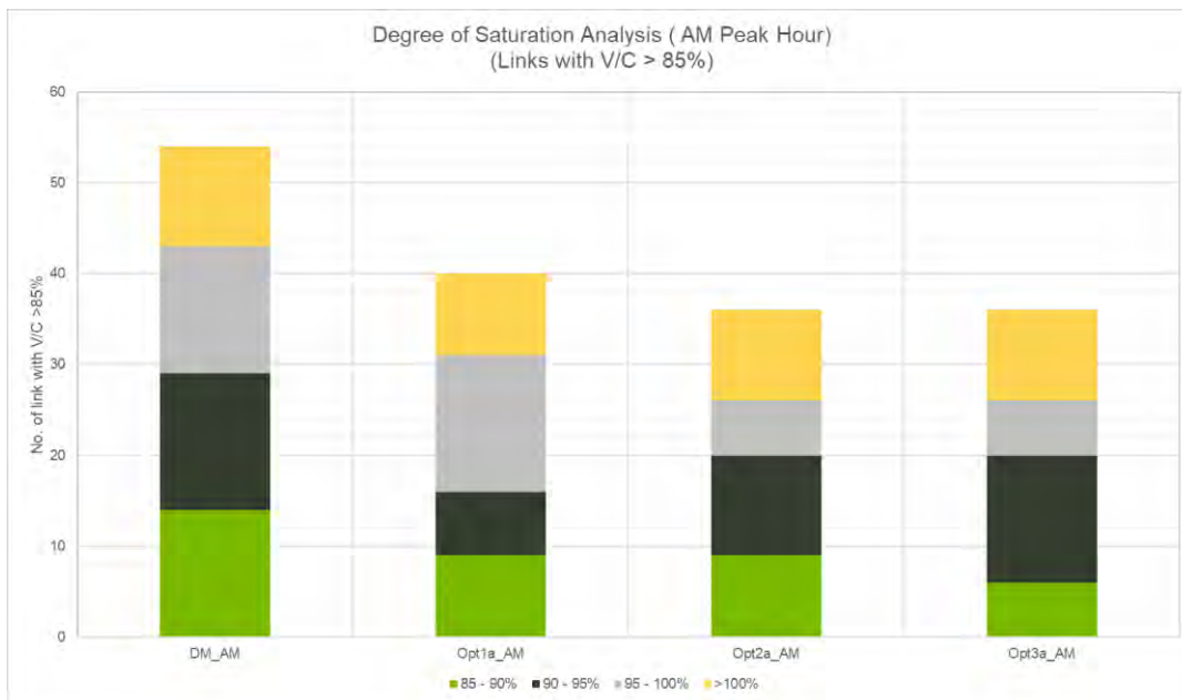
Figure 7: Degree of saturation assessment (AM peak)
