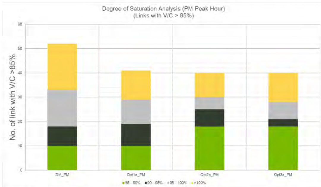
Figure 9: Degree of saturation assessment (PM peak)
