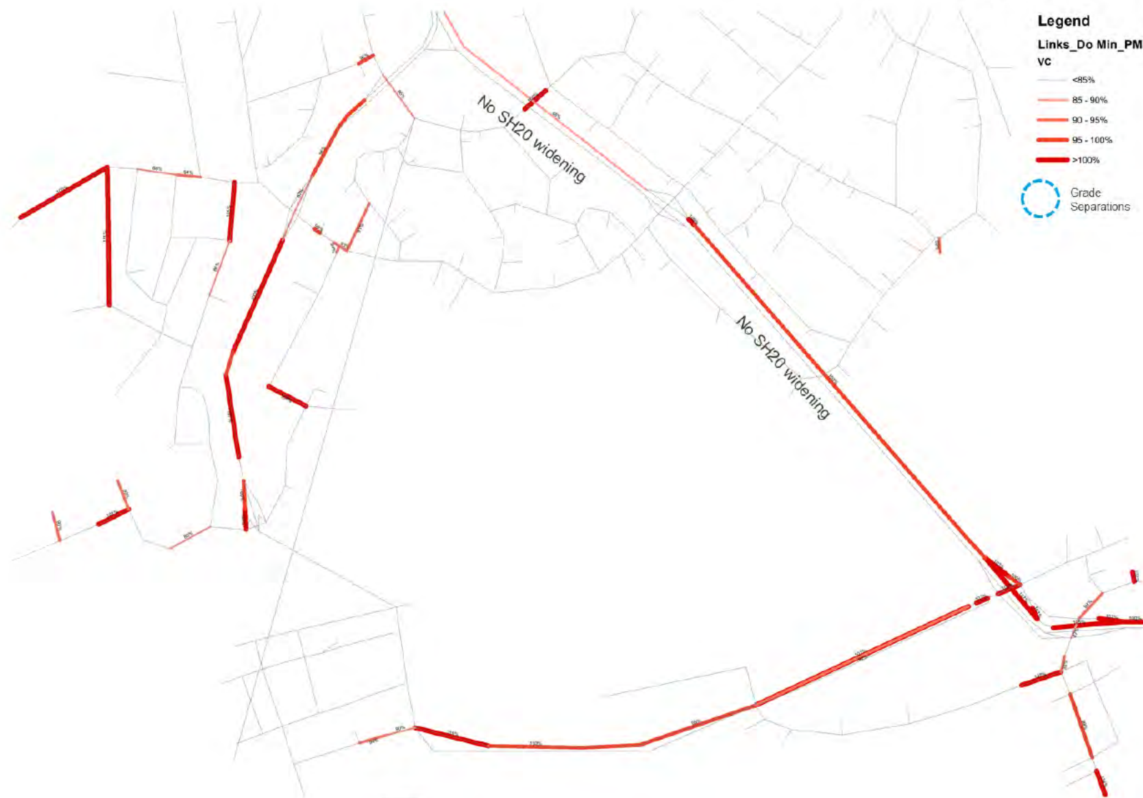
Figure 10: Degree of saturation – Do Minimum (PM peak)
