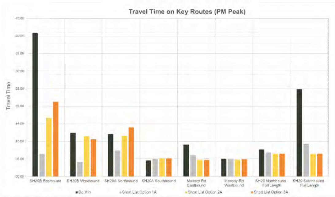
Figure 18: Travel times on key routes (PM Peak)
