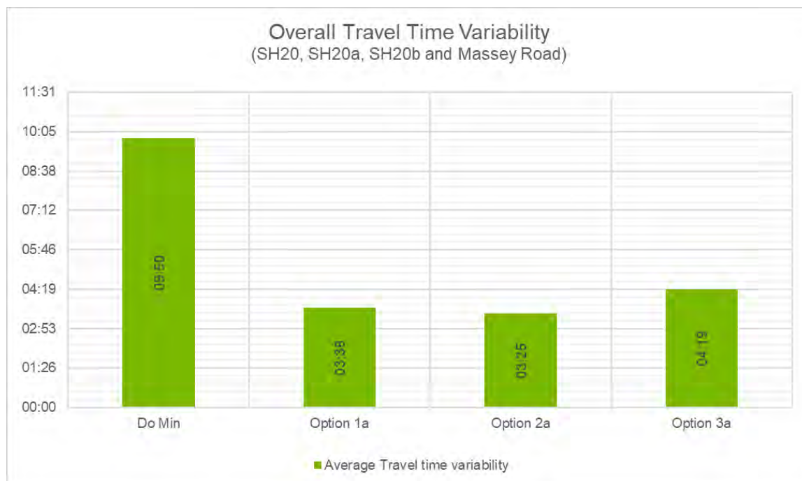
Figure 14: Average travel time variability of key routes for each option (SATURN)
