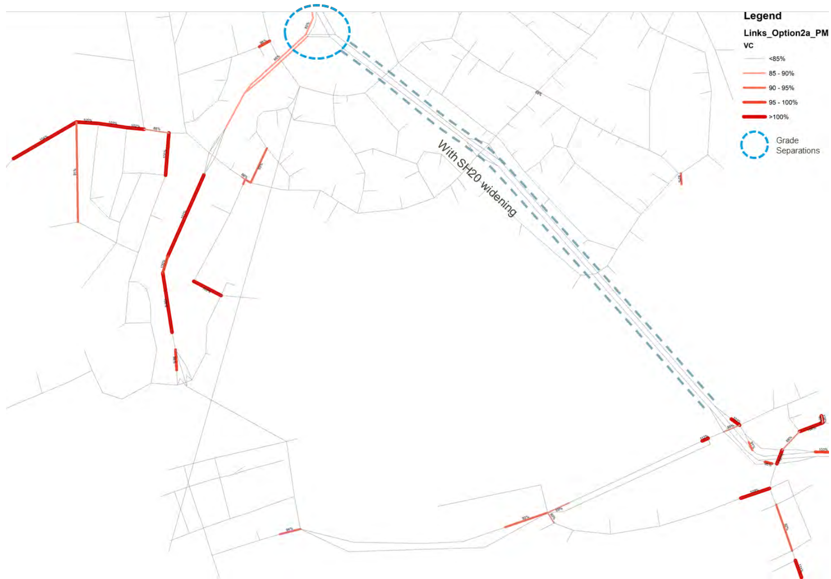
Figure 12: Degree of saturation - Option 2A (PM peak)
