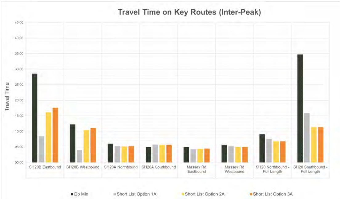
Figure 17: Travel times on key routes (inter-peak)
