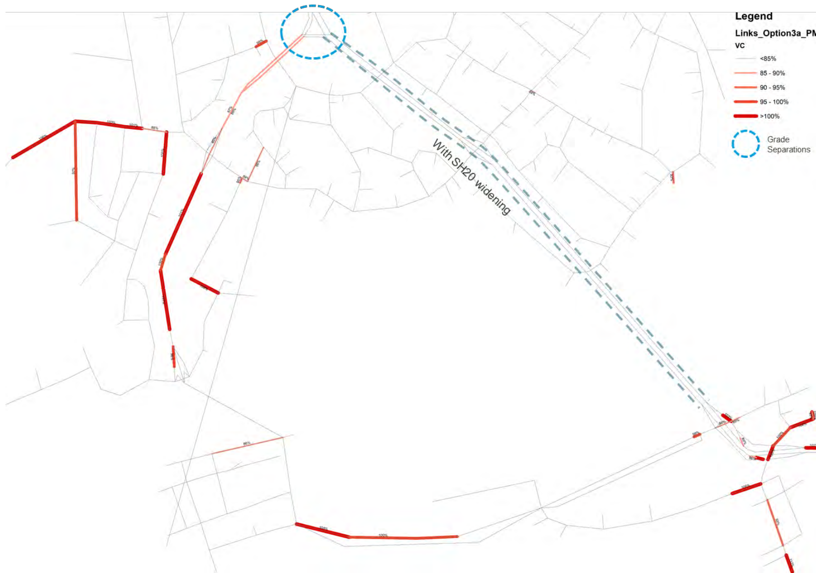
Figure 13: Degree of saturation - Option 3A (PM peak)
