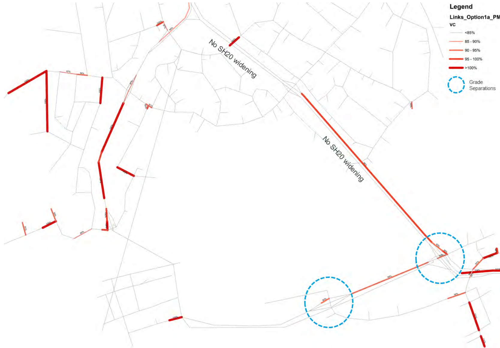
Figure 11: Degree of saturation - Option 1A (PM peak)
