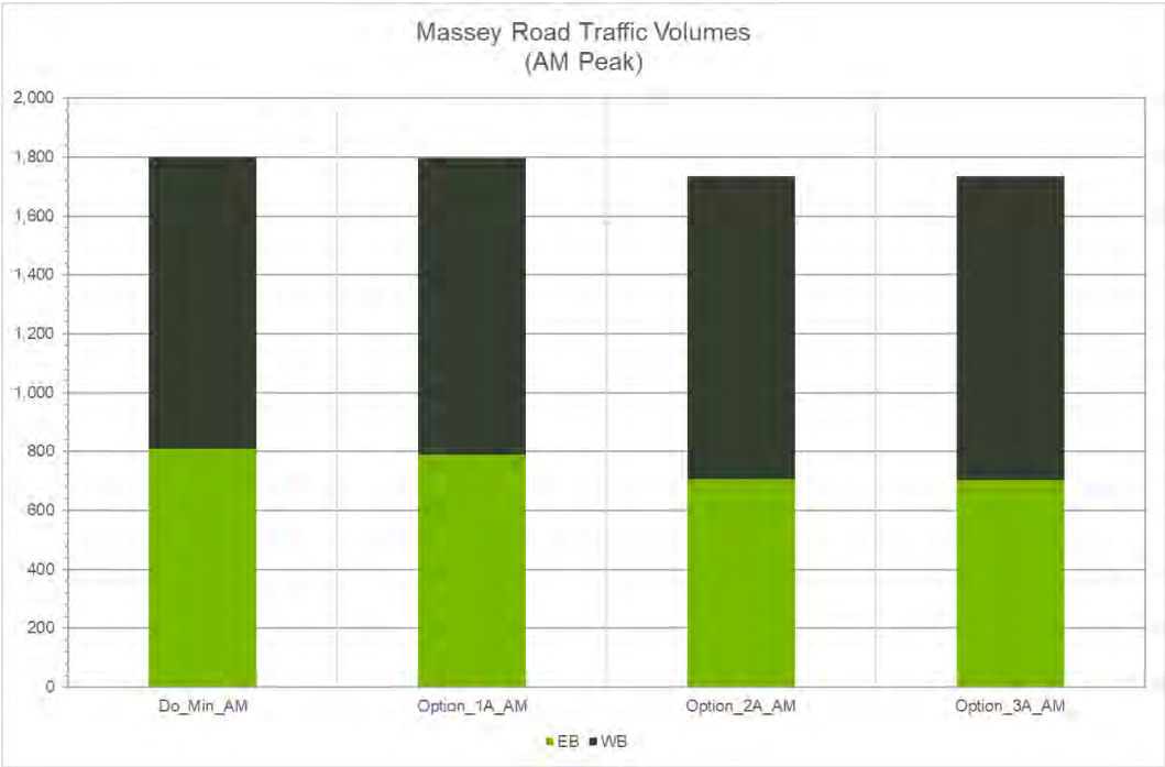
Figure 23: Massey Road traffic volumes (AM peak, 2048)
