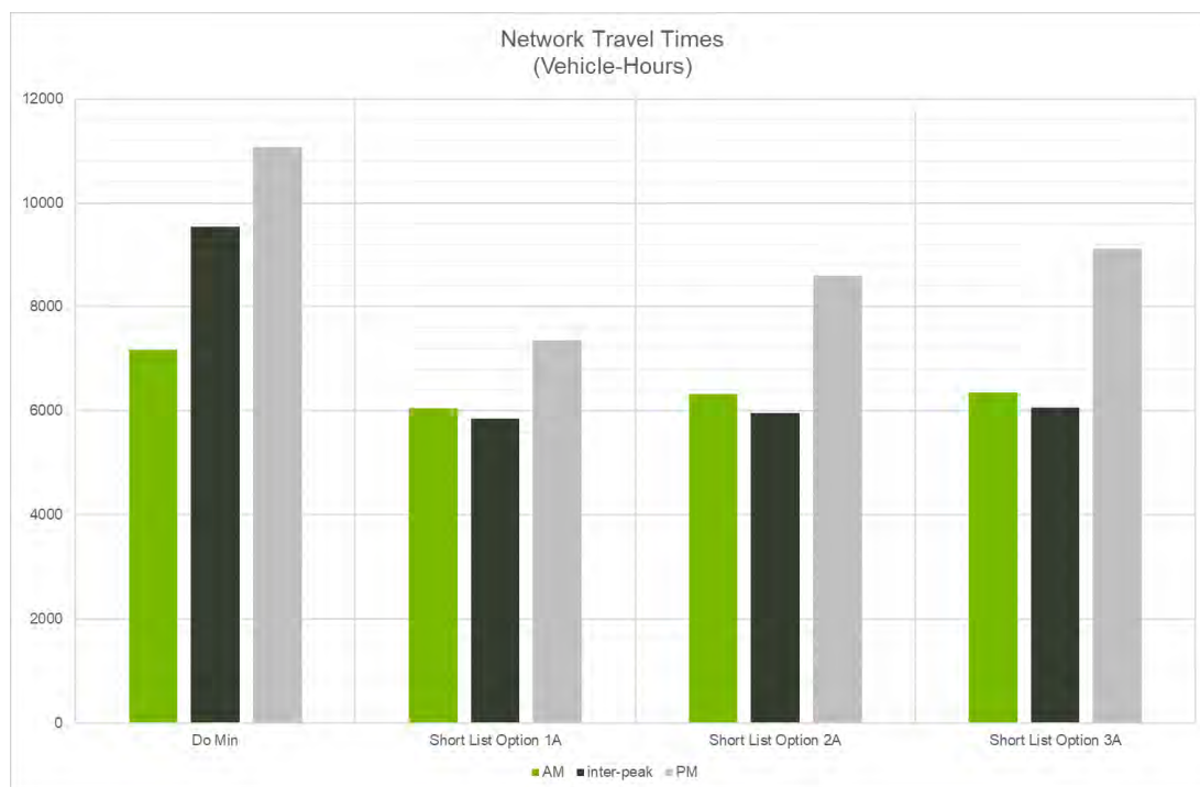
Figure 15: Overall network travel times (vehicle-hours)
