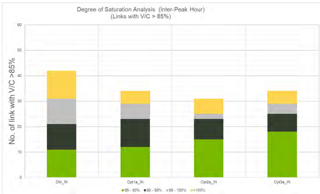
Figure 8: Degree of saturation assessment (inter-peak)
