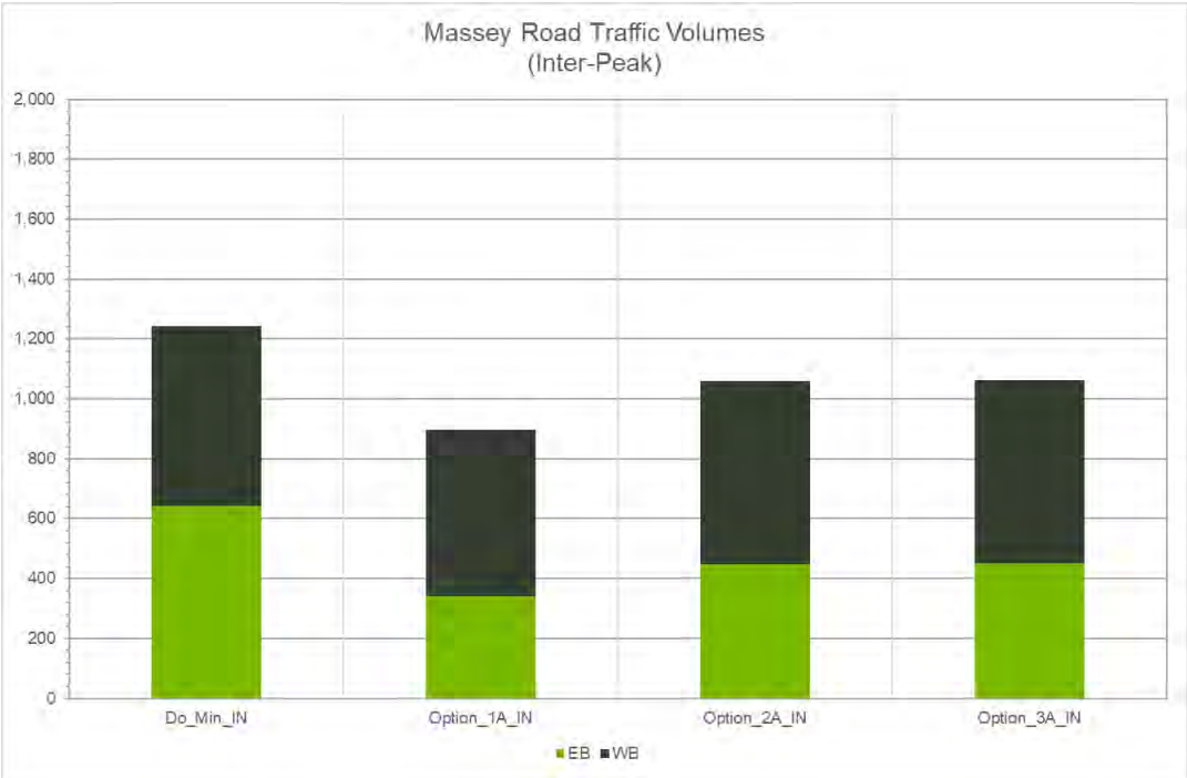
Figure 24: Massey Road traffic volumes (Inter-peak, 2048)
