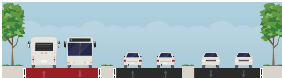
Figure 14-3: A-side running RTC route, the preferred placement for the Davies Avenue and SH20B section of the A2B corridor
