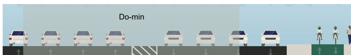
Figure 15-30: Proposed SH20 north of SH20A cross-section
