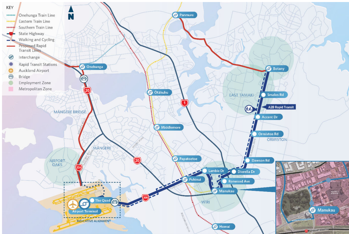
Figure 15-14: A2B route, stations and interchanges
