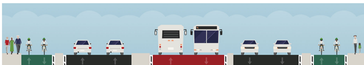
Figure 15-33: A2B Te Irirangi Drive typical cross-section
