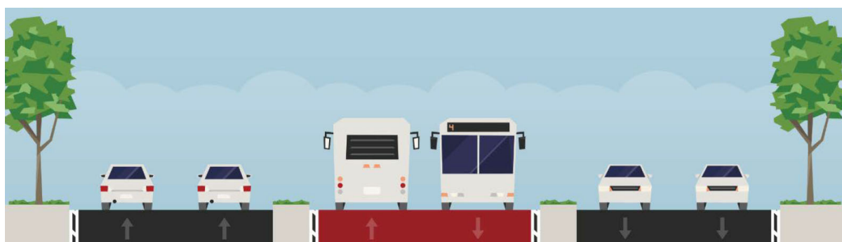
Figure 14-2: Central-running RTC route, preferred for most of the A2B corridor
