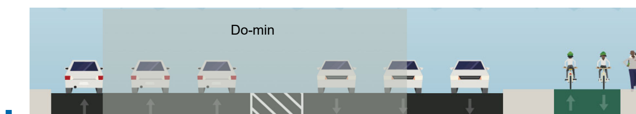
Figure 15-31: Proposed SH20 between SH20A and SH20B cross-section
