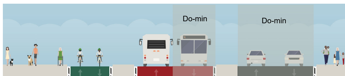
Figure 15-9 A2B cross-section - Davies Avenue
